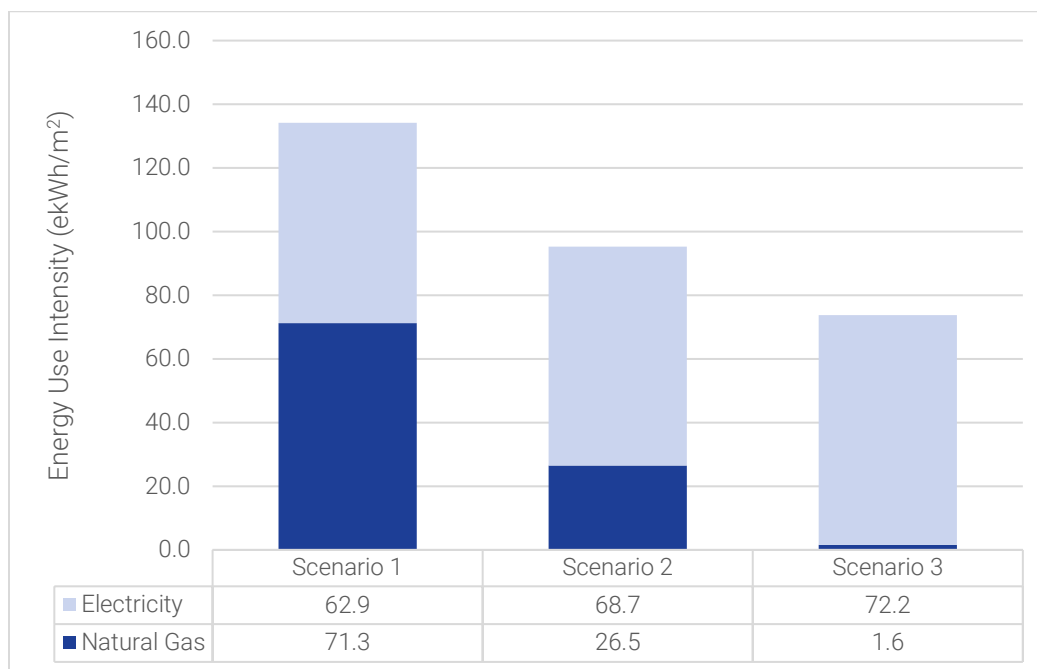
Figure 3 - Predicted Energy Consumption by End-Use
