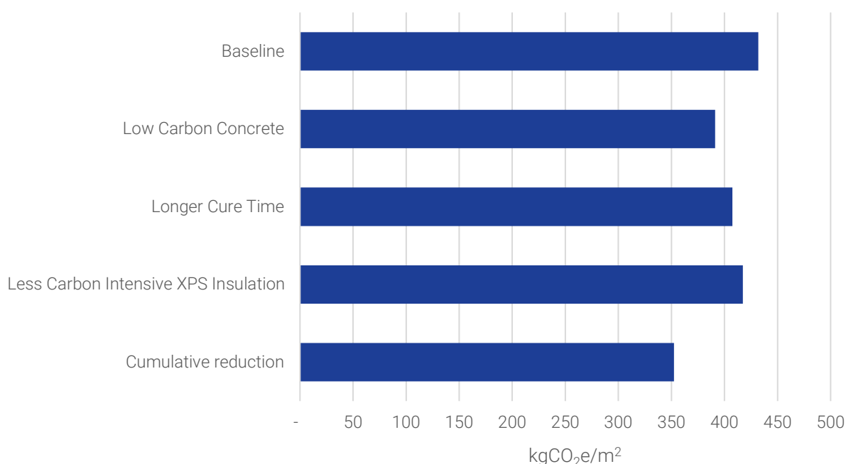
Figure 19– Embodied Carbon Reduction Summary Graph
