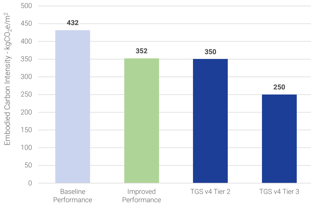
Figure 20 - Estimated Embodied Carbon Benchmarked Performance
