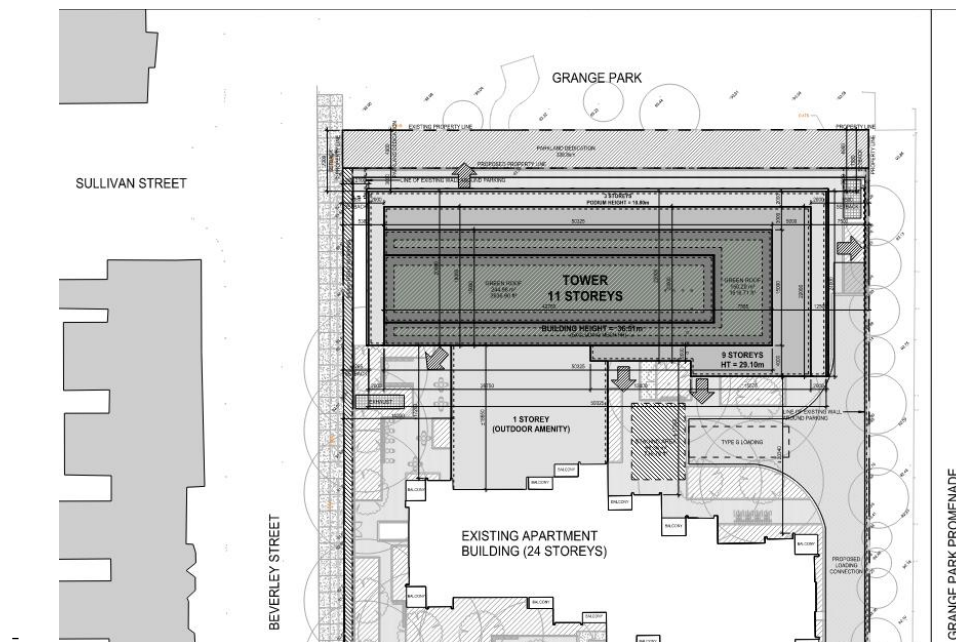
Figure 1 – Proposed Development Concept Plan 1
