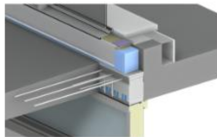
High performing detail – Thermally Broken Balcony System 17
