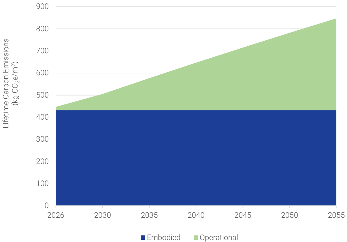
Figure 14 - Embodied versus Operational Carbon
