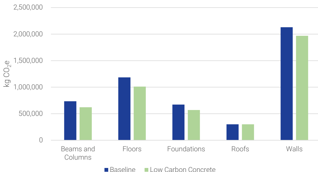
Figure 18 – Low Carbon Concrete – 30-40% SCM and GUL
