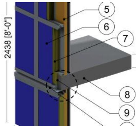
Low performing detail – Window-wall, slab edge with firestop insulation 12
